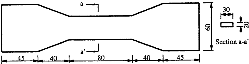
FIG. 1. Shape and dimensions (in mm) of the specimens tested under tension.
